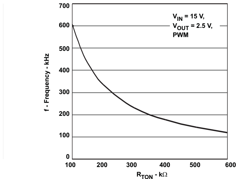
Figure 1. Switching Frequency vs R_{TON}
