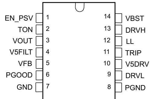
TSSOP (PW) PACKAGE (TOP VIEW)
