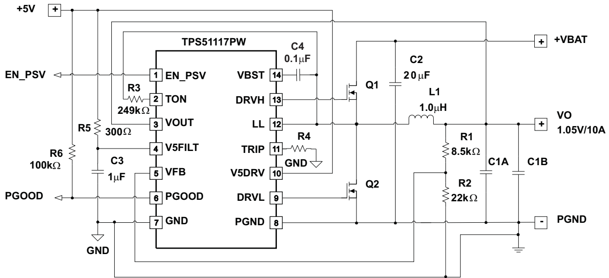
Figure 23. 1.05-V/10-A Application From VBAT (PW Package)
