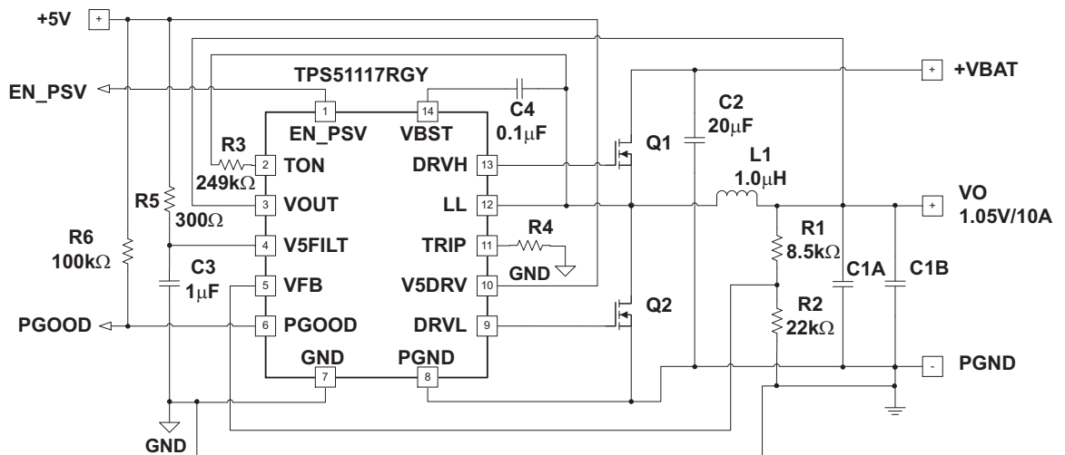
Figure 24. 1.05-V/10-A Application From VBAT (RGY Package)
